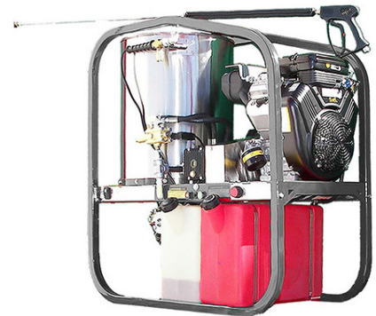
LTK Series Pressure Washer
